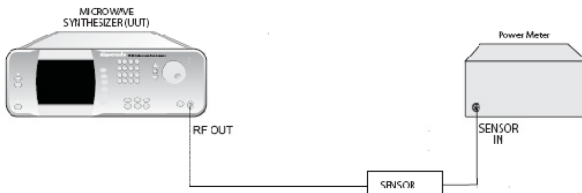
Figure 50. Power Specifications Test Setup
