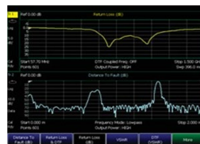
View return loss and DTF simultaneously
